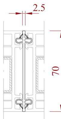
Accouplement vertical 109.346
